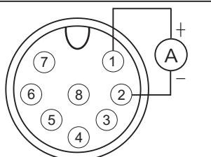
Power wiring connection for RS-485
