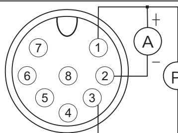
Wiring connection
