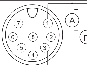
Wiring connection
